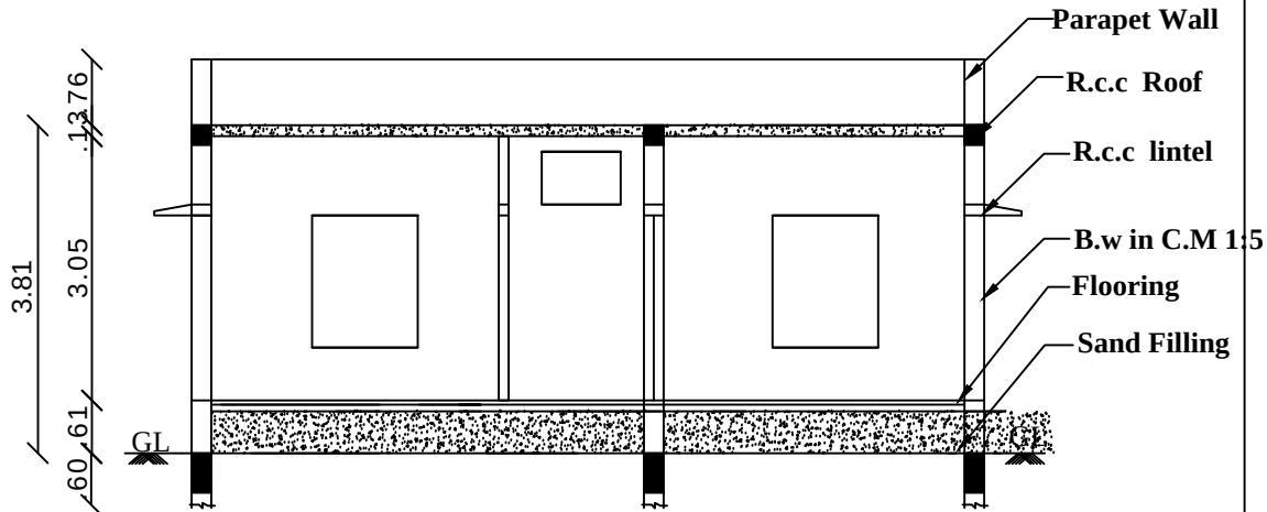
SECTION-AB
