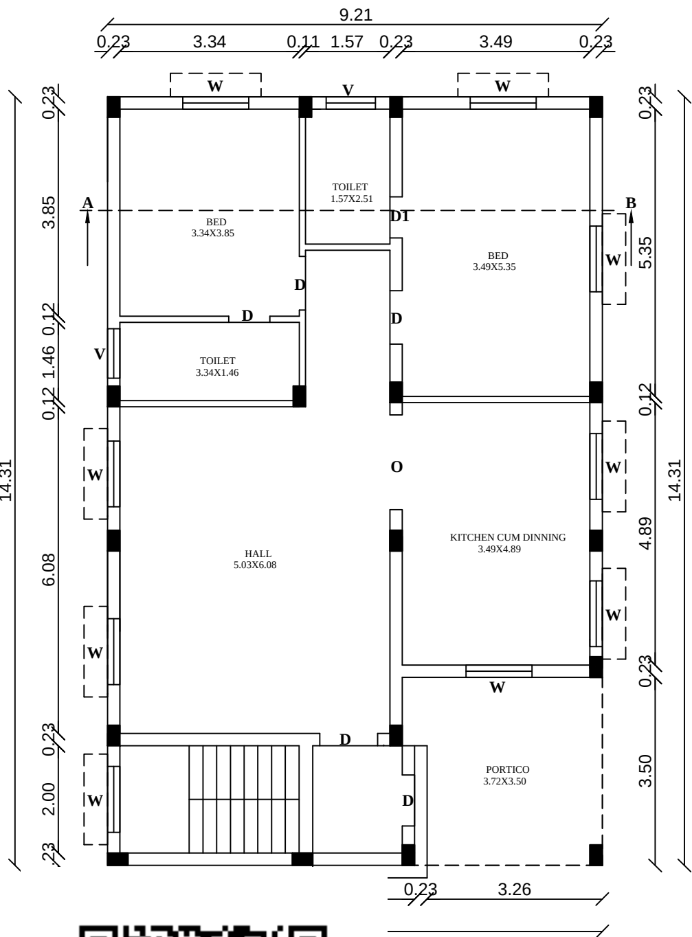
FLOOR PLAN
