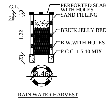
RAIN WATER HARVEST
