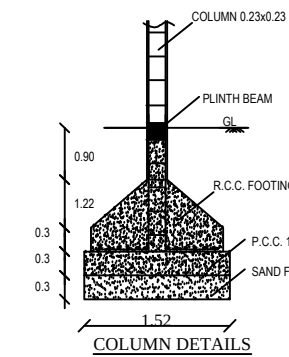
COLUMN DETAILS
