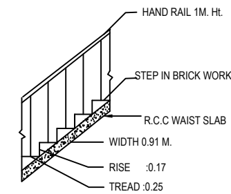
STAIR DETAIL
