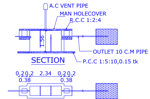
PLAN OF SEPTIC TANK & TRENCH
