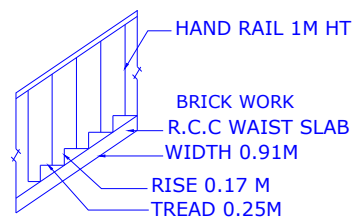
STAIRCASE DETAIL
