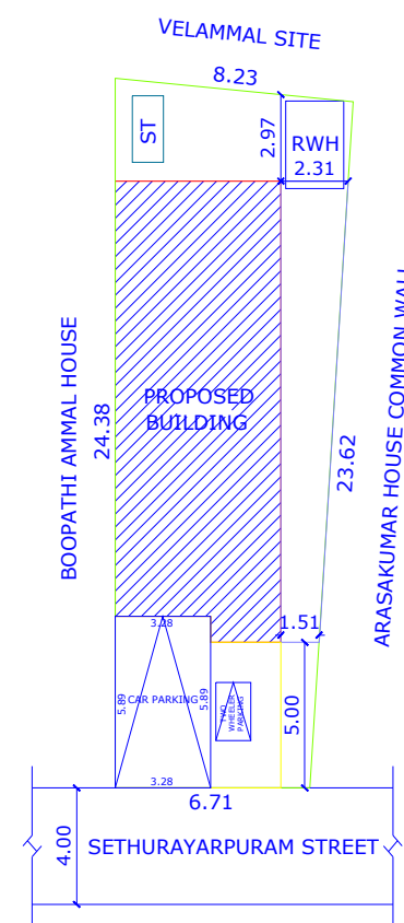
SITE PLAN SCALE - 1:200
