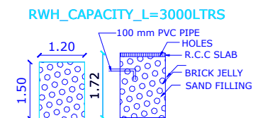
PLAN & SECTION OF RAIN WATER COLLECTION TANK
