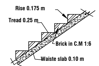
STAIR DETAILS
