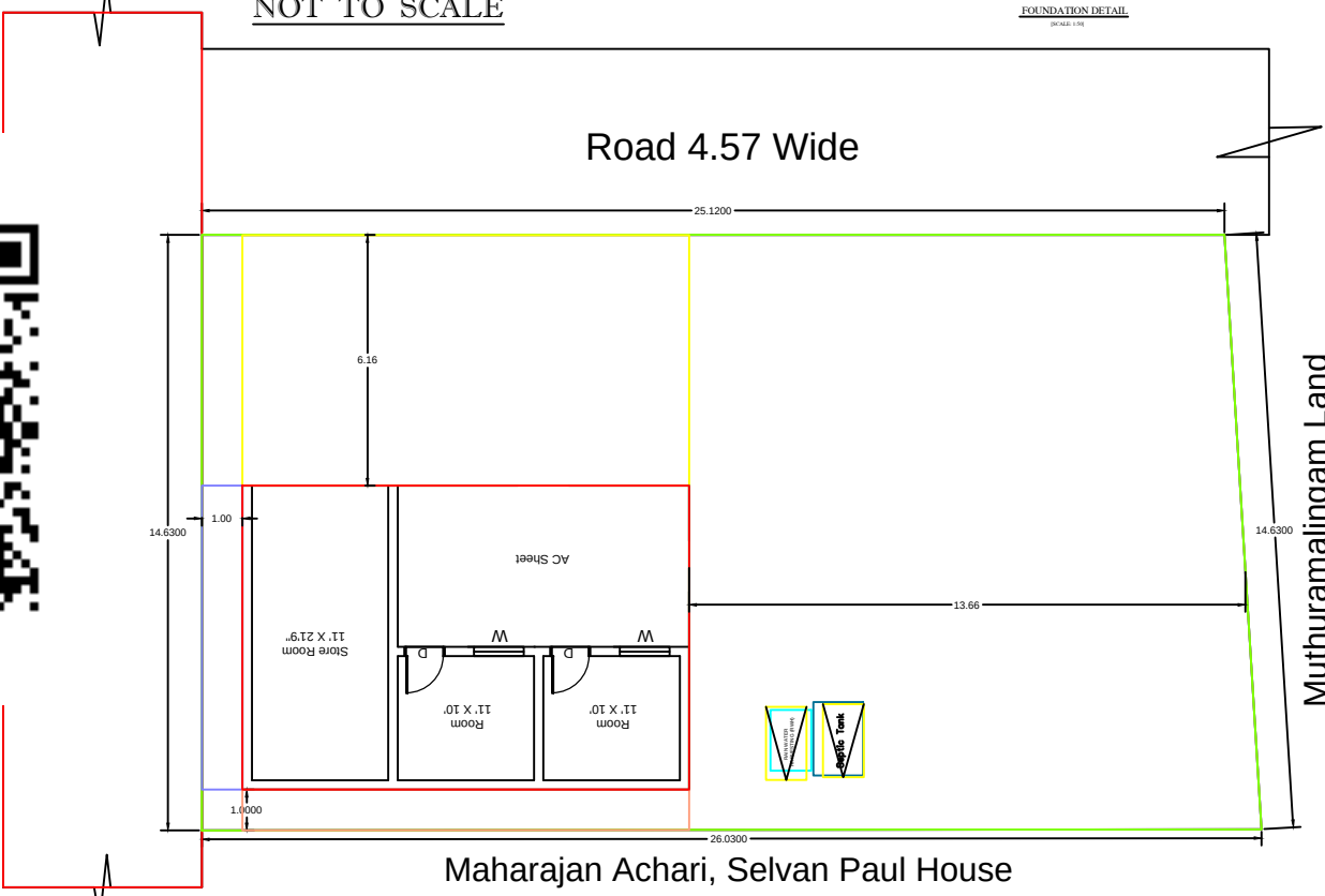
FOUNDATION DETAIL (NOT FOR SCALE)
