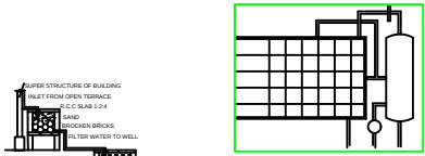
RAINWATER HARVESTING
