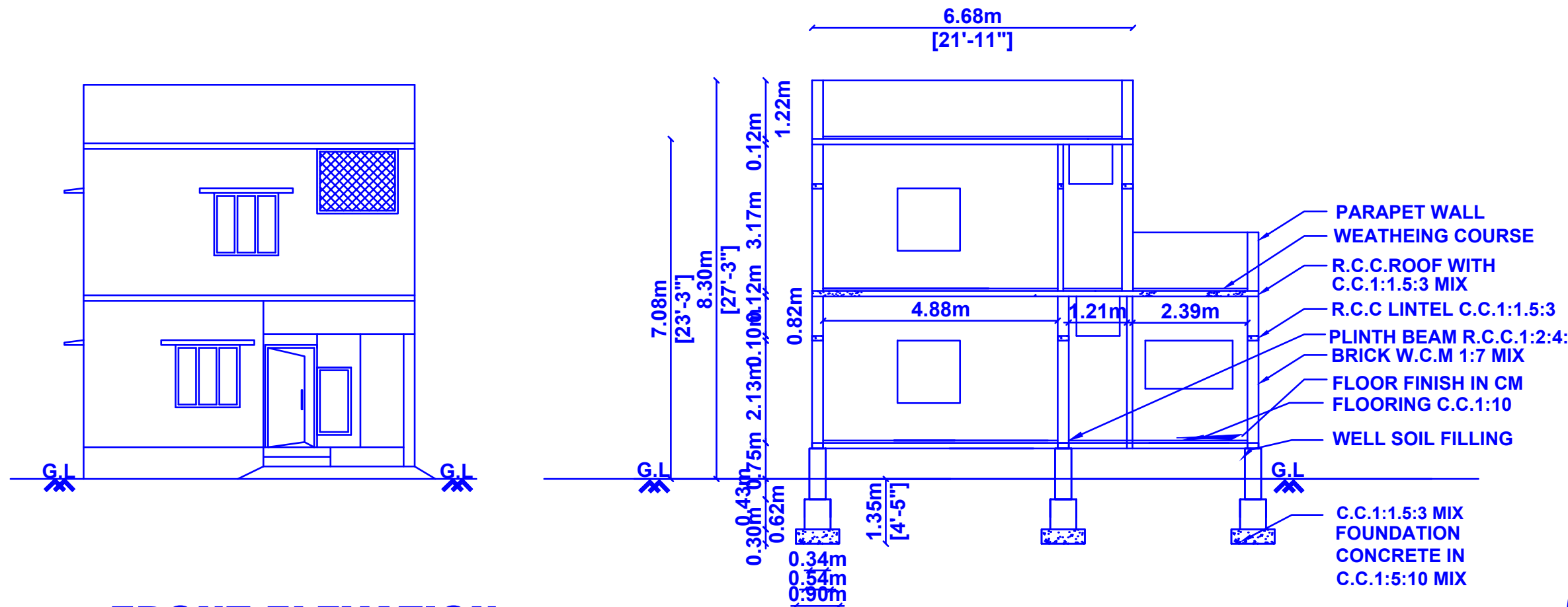
FRONT ELEVATION
