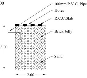
SECTION OF RAIN WATER COLLECTING TANK
