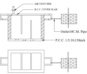
Exi. Septic Tank and Trench
