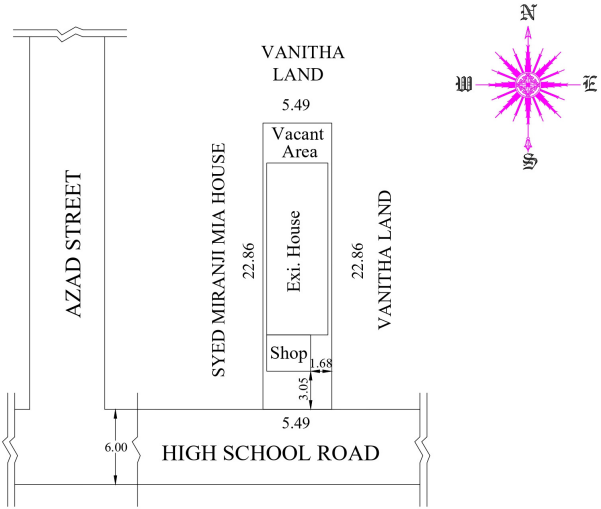
SITE PLAN
