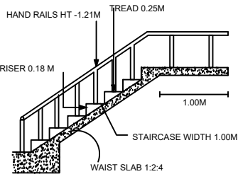
STAIRCASE DETAILS
