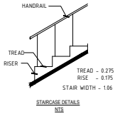
STAIRCASE DETAILS
