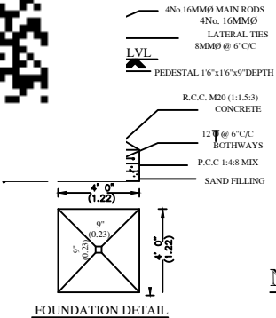
FOUNDATION DETAIL
