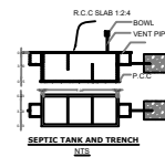
SEPTIC TANK AND TRENCH
