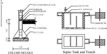
COLUMN DETAILS
