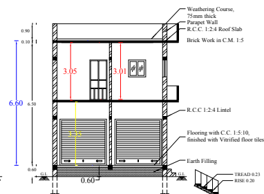
SECTION A - B
