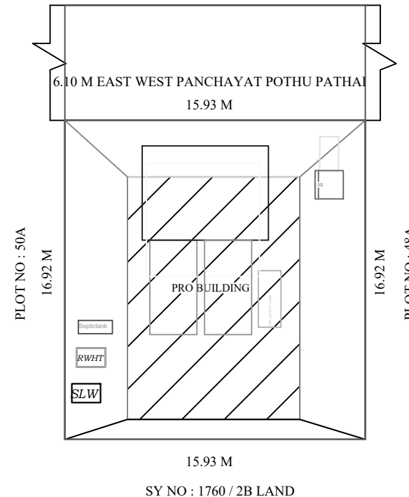
SITE PLAN
