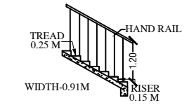
STAIRCASE DETAILS
