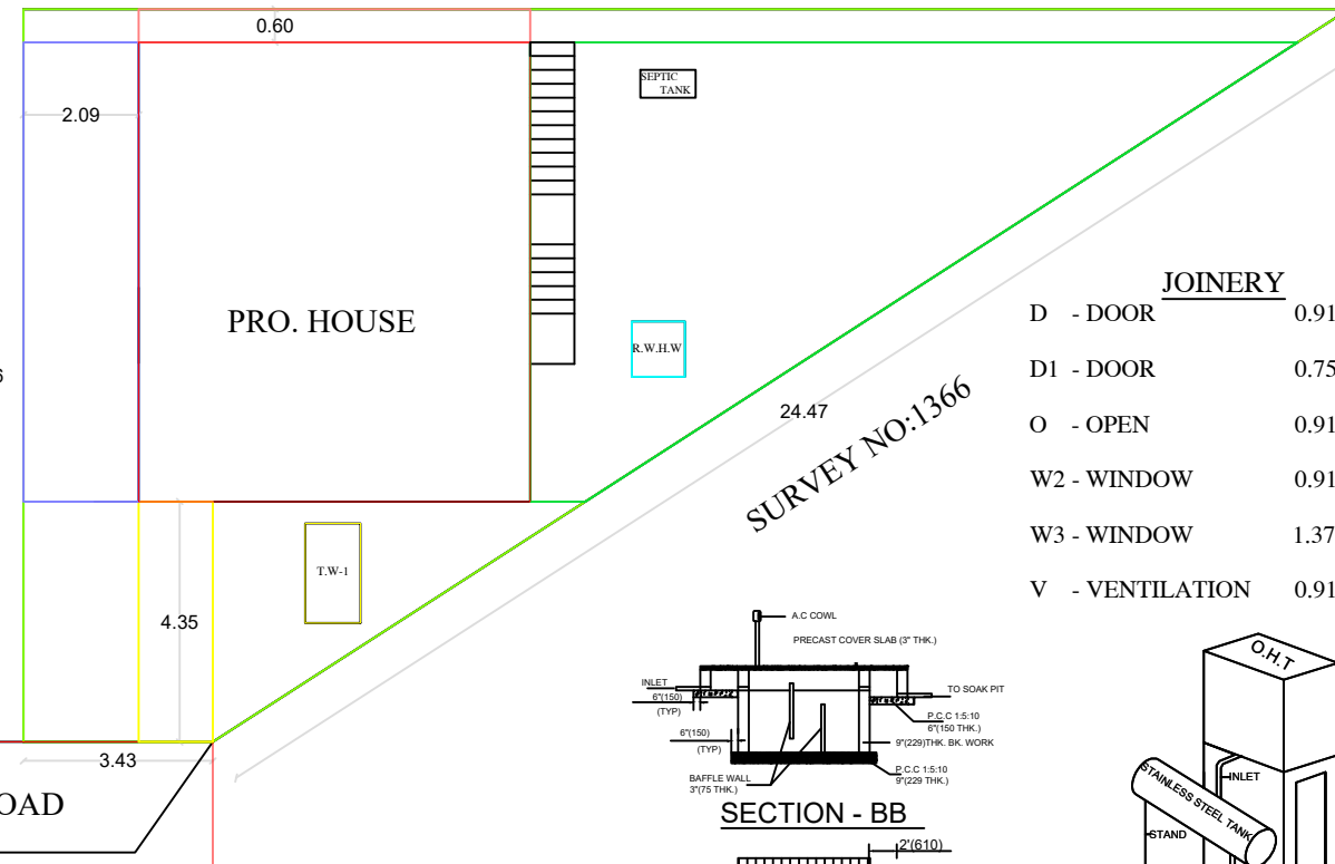
SITE PLAN
