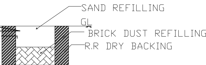
DETAILS OF RAIN WATER HARVESTING
