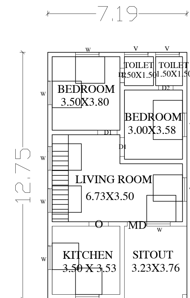
GROUND PLAN
