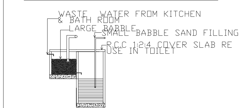
RECYCLING OF WASTE WATER FROM KITCHEN & BATHROOM
