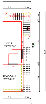
R PLAN
