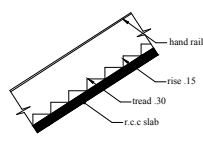
Stair
