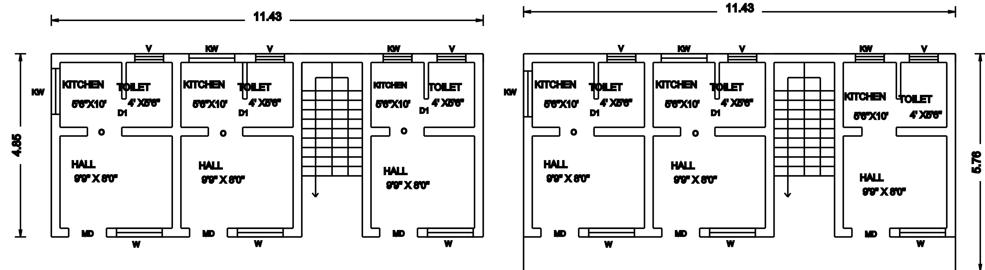
PRO.GROUND FLOOR PLAN
