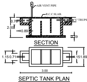
SECTION SEPTIC TANK PLAN
