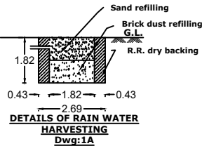
DETAILS OF RAIN WATER HARVESTING Dwg:1A
