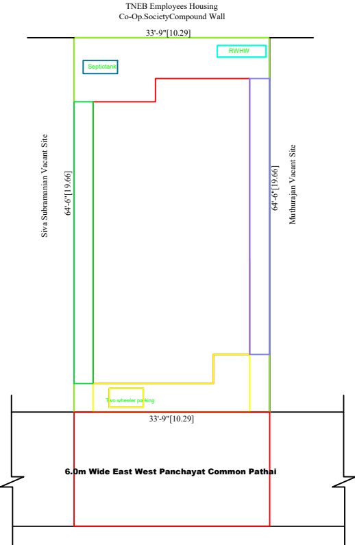
SITE PLAN
