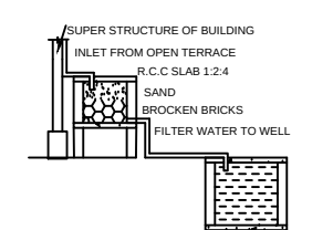
RAINWATER HARVESTING
