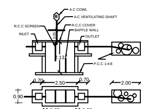
SEPTICTANK DETAILS
