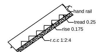
STAIR
