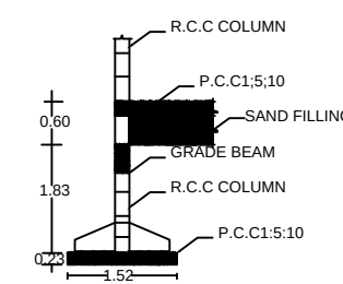
COLUMN DETAILS
