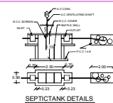
SEPTICTANK DETAILS
