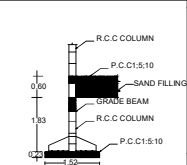
COLUMN DETAILS
