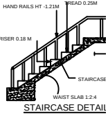
STAIRCASE DETAIL
