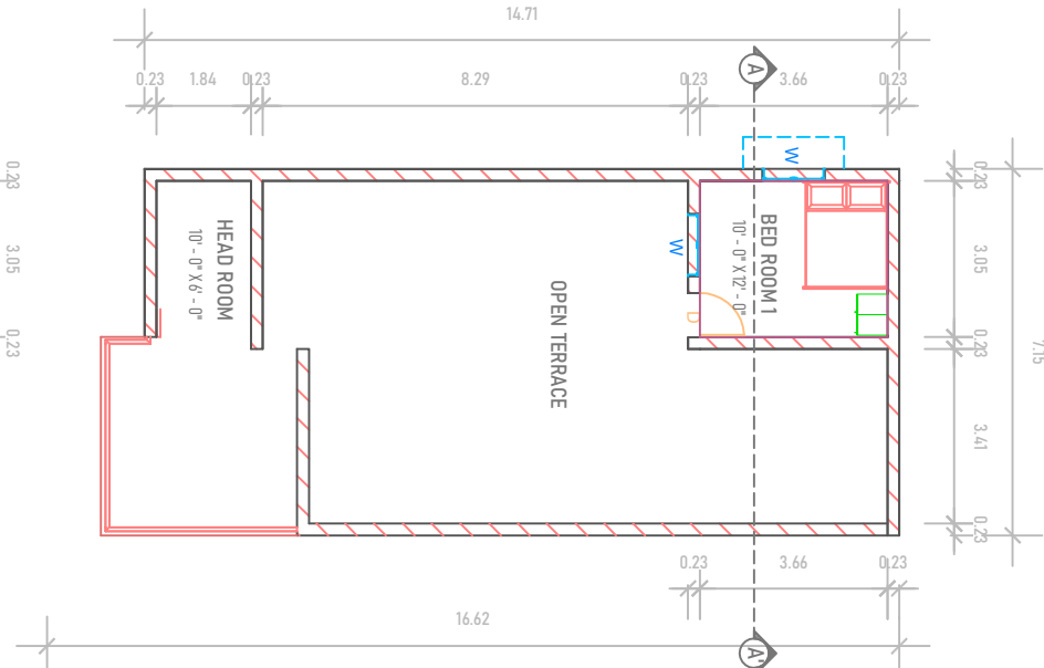
PRO FIRST FLOOR
