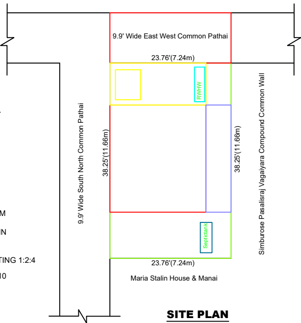
SITE PLAN
