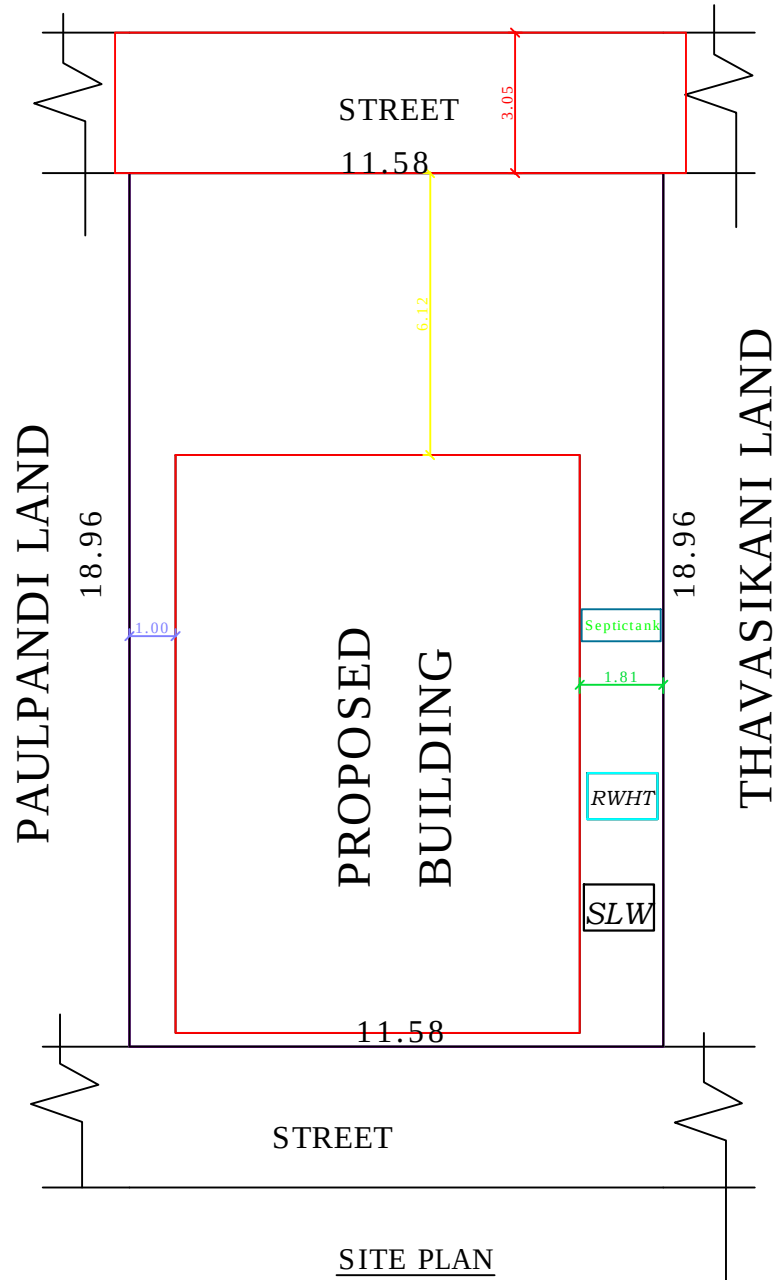
SITE PLAN
