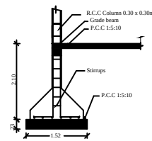
Column Detail
