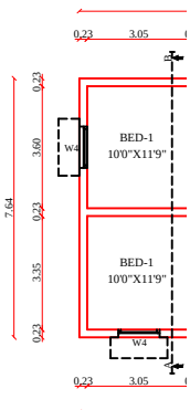
GROUNDFLOOR PLAN
