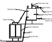
Details Of Solar Water Heater (NTS)
