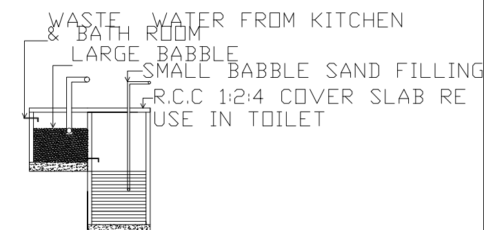
RECYCLING OF WASTE WATER FROM KITCHEN & BATHROOM
