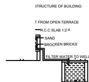
DETAILS OF FILTER BED & WELL NTS
