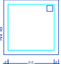
DETAILS OF COLLECTION SUMP FOR RAIN
