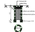
PERCOLATION PIT FOR 30 Sq. ft. (Scale:- 1:50)
