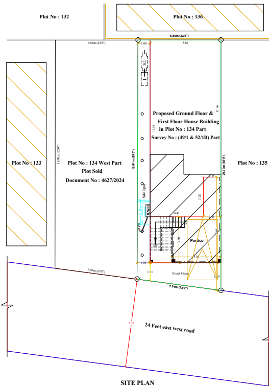
SITE PLAN
