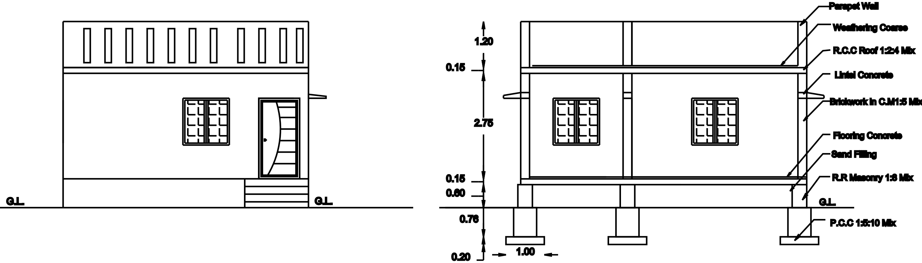
FRONT ELEVATION
