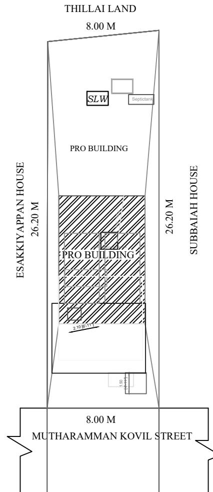
SITE PLAN
