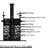
DETAILS OF R.C.C. COLUMN
