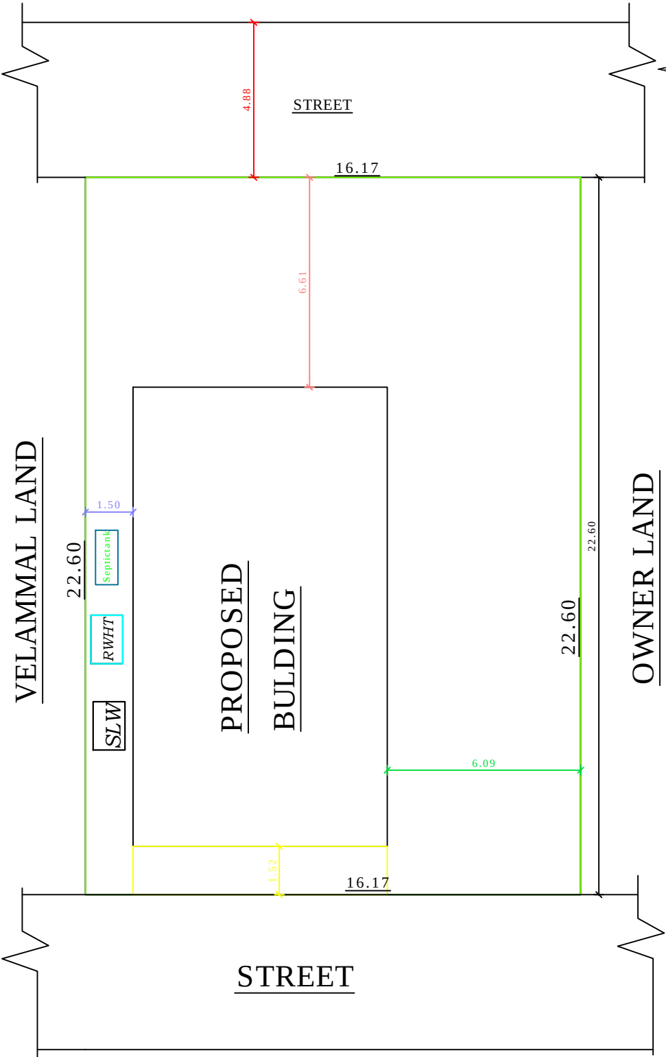
SITE PLAN
