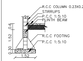
COLOUMN DETAILS
