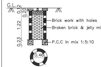
PERCOLATION PIT FOR 30 Sq. m. (Scale: - 1:50)
