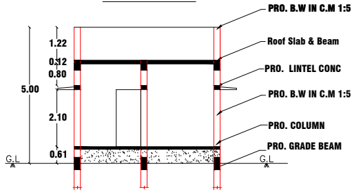
CROSS SECTION ON XX
