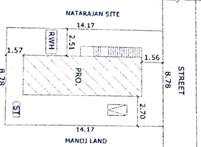
TOPO PLAN SCALE - NOT TO SCALE
