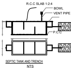
SEPTIC TANK AND TRENCH NTS
