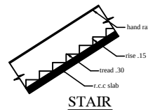
STAIR
