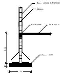
Column Detail
