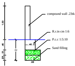
Compound Wall Detail
