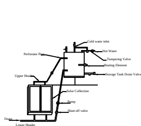
Details Of Solar Water Heater (NTS)
