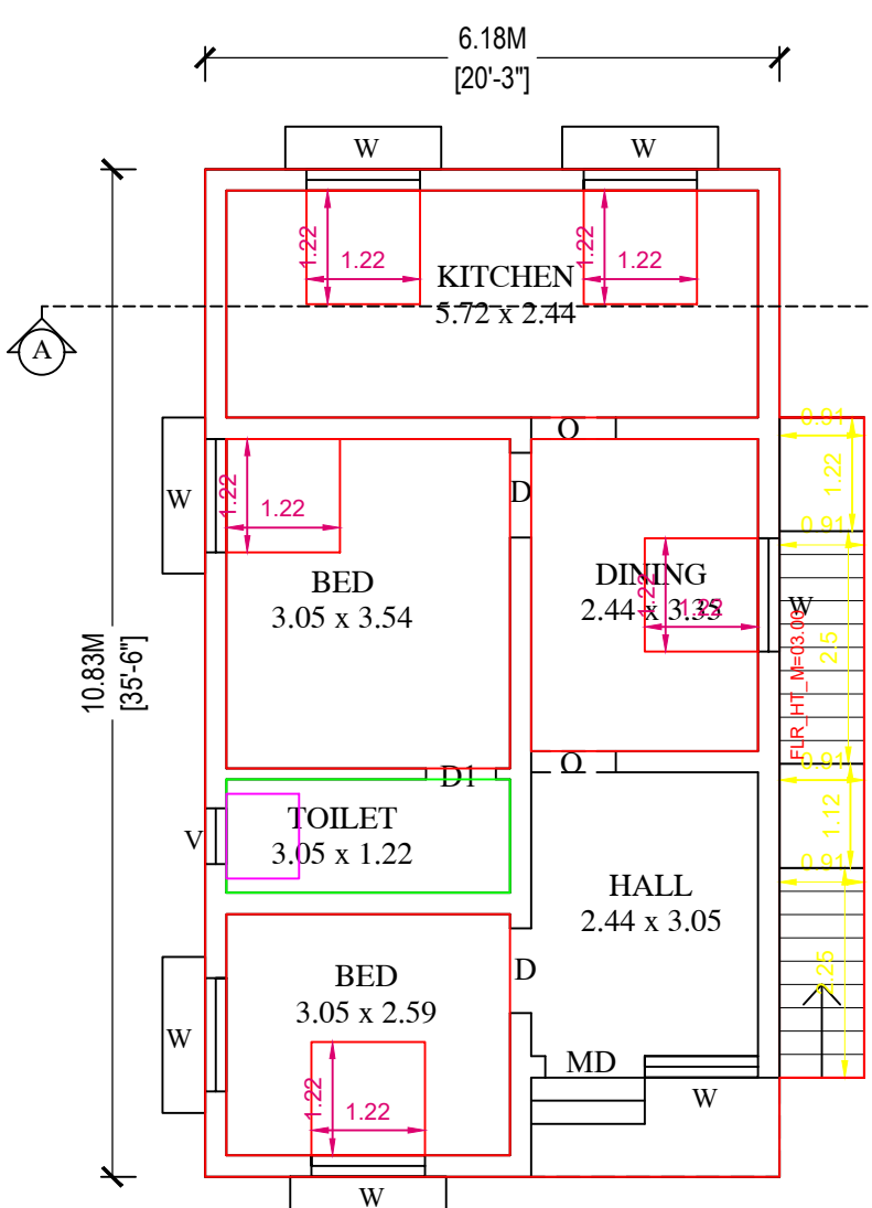
PRO.GOUND FLOOR PLAN
