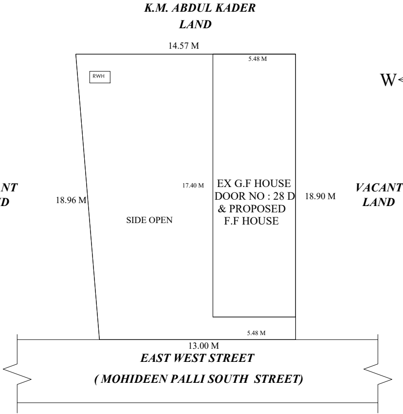
SITE PLAN
