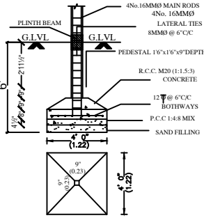
FOUNDATION DETAIL
