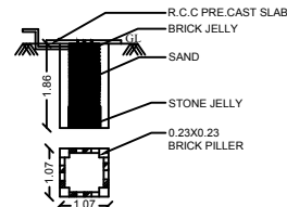
PLAN AND SECTION OF RAINWATER COLLECTION WELL
