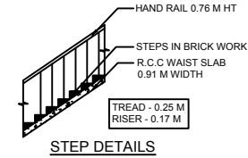
STEP DETAILS
