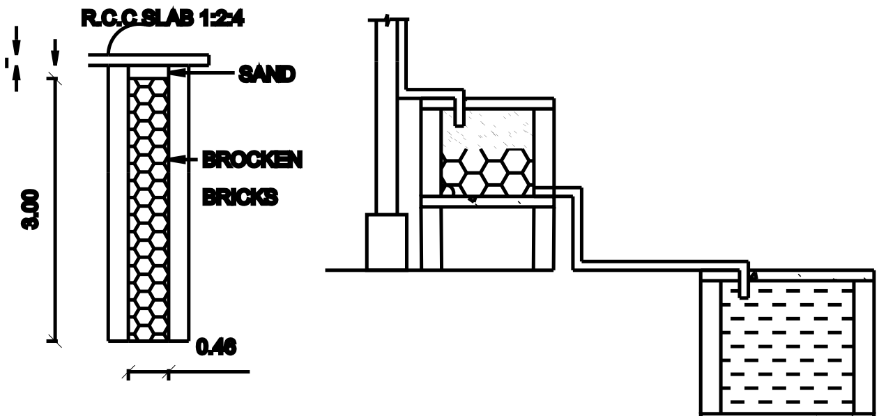
DETAILS OF FILTER BED & WELL
