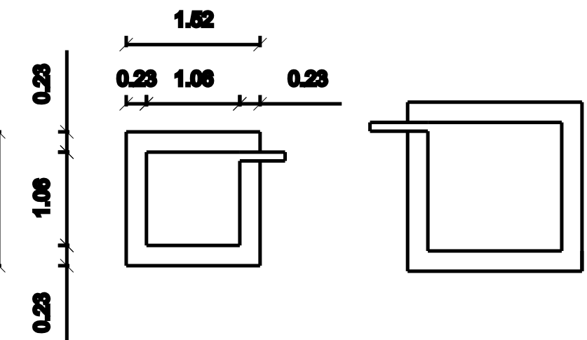
DETAILS OF FILTER BED & WELL
