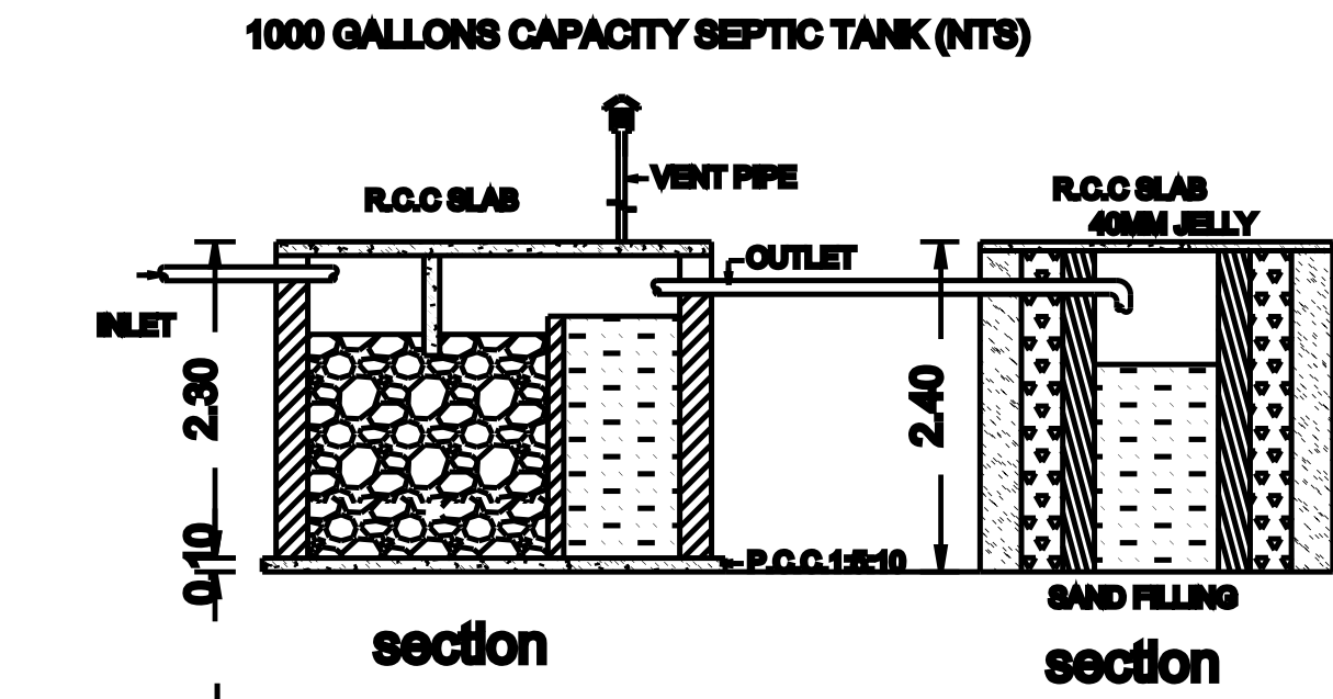
section
