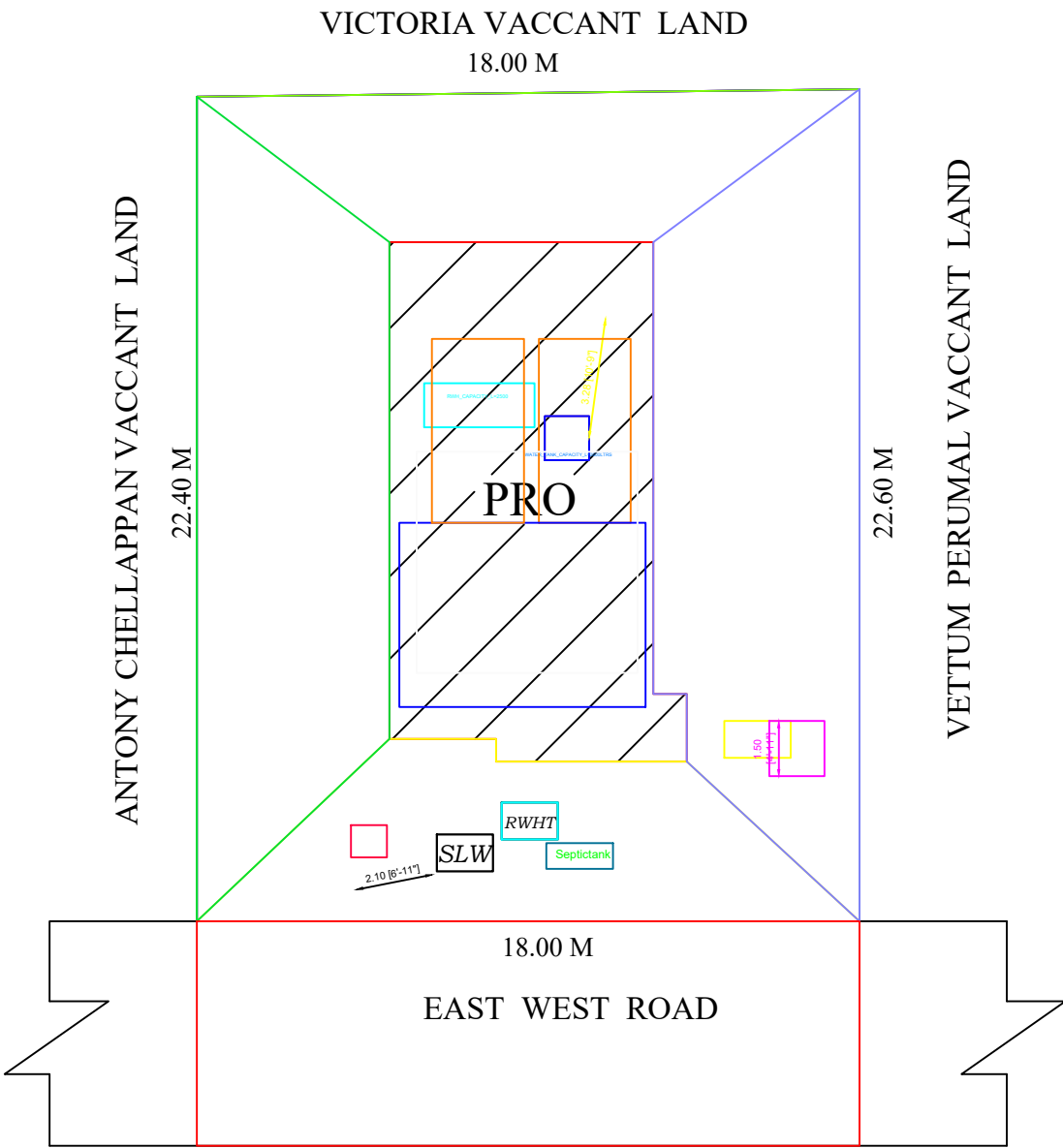
SITE PLAN
