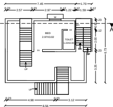
PRO.FIRST FLOOR PLAN
