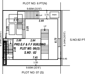
SITE PLAN
