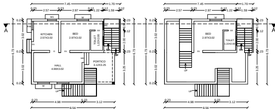
PRO. GROUND FLOOR PLAN
