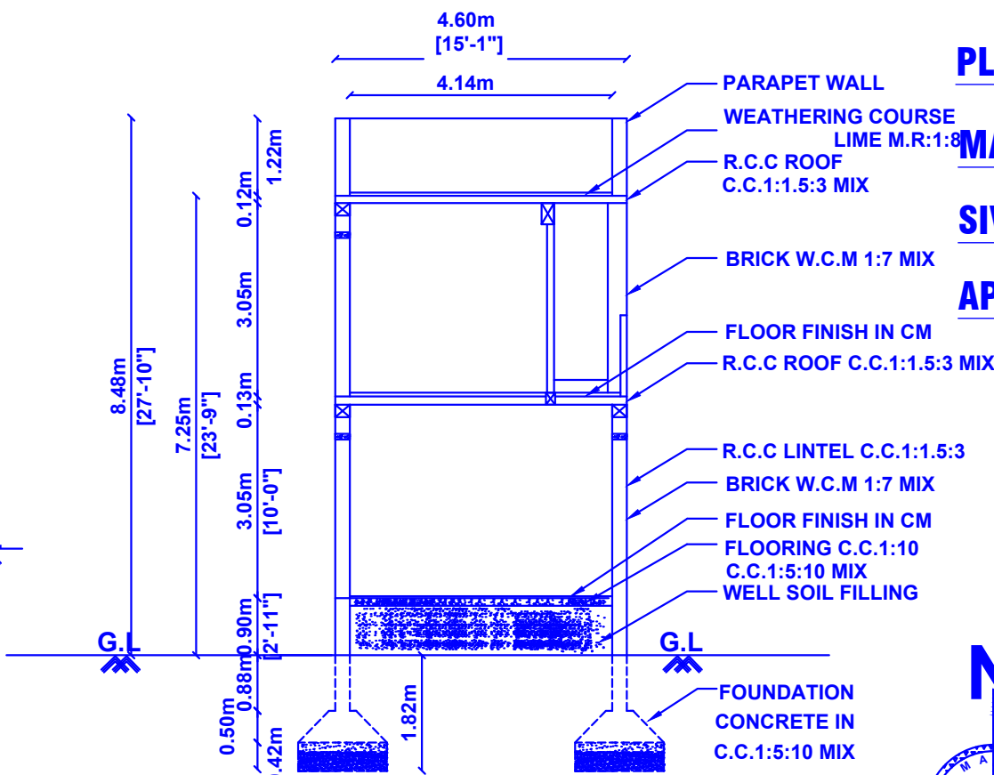
SECTION ON "G1-G2"
