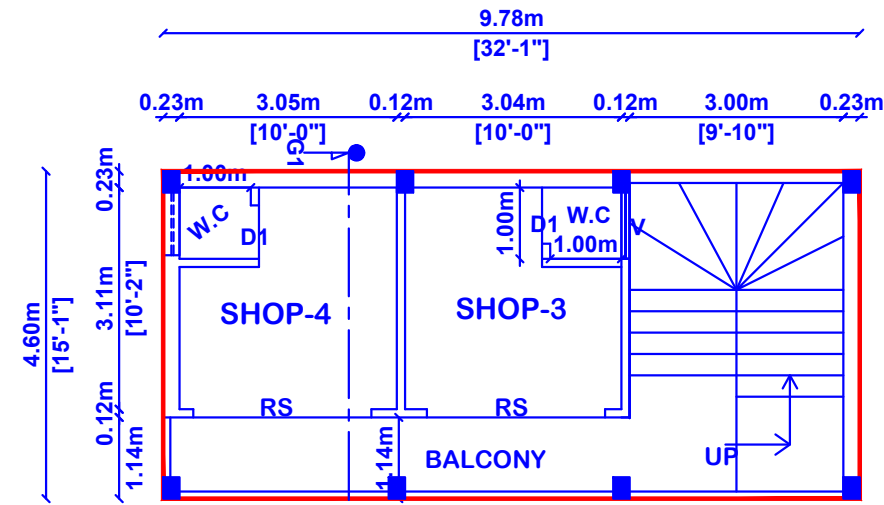
FIRST FLOOR PLAN (Proposed)
