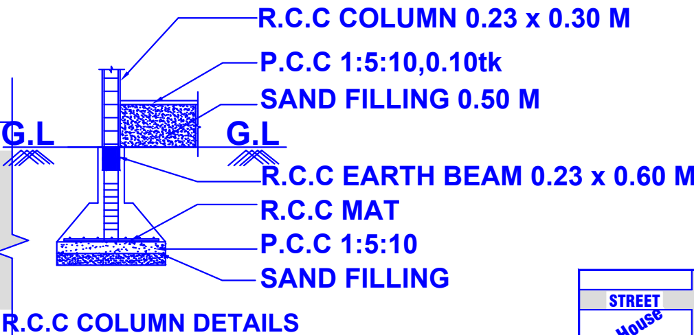
R.C.C COLUMN DETAILS
