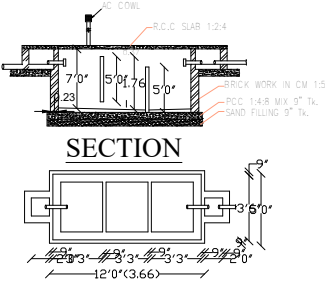
SECTION PLAN SEPTIC TANK DETAILS
