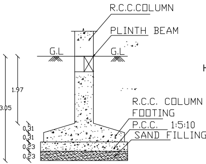
FOUNDATION DETAIL
