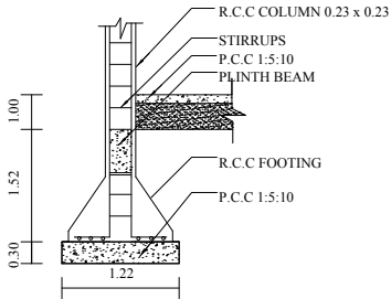
COLUMN DETAILS
