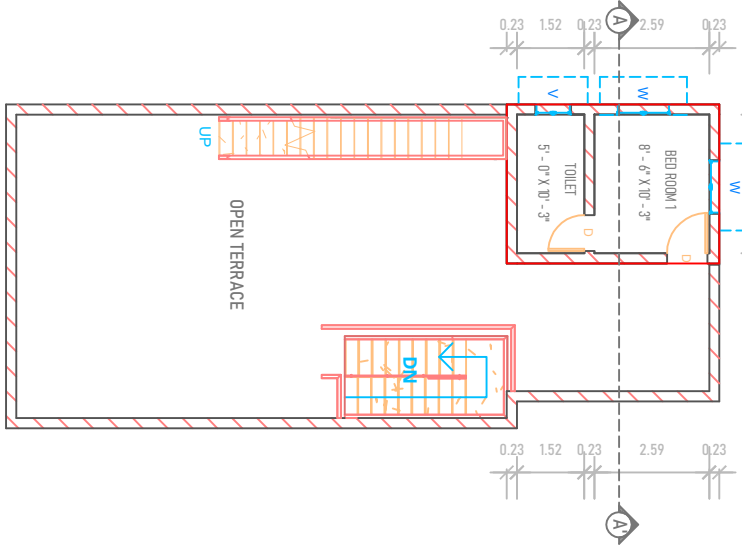
PRO FIRST FLOOR
