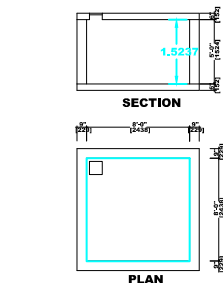
DETAILS OF COLLECTION SUMP FOR RAIN WATER HARVESTING OF ROOF TOP RAIN WATER RWH_CAPACITY_L=5000LTRS
